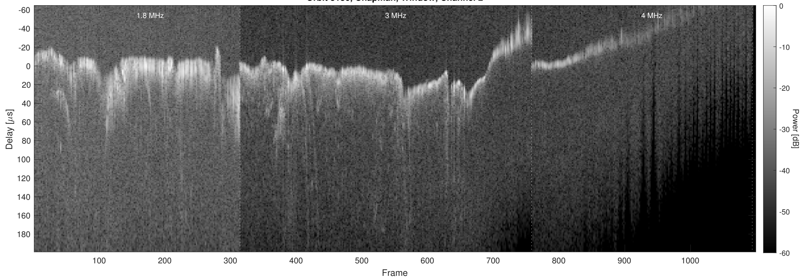
Orbit 8186, Chapman, Window, Channel 2
