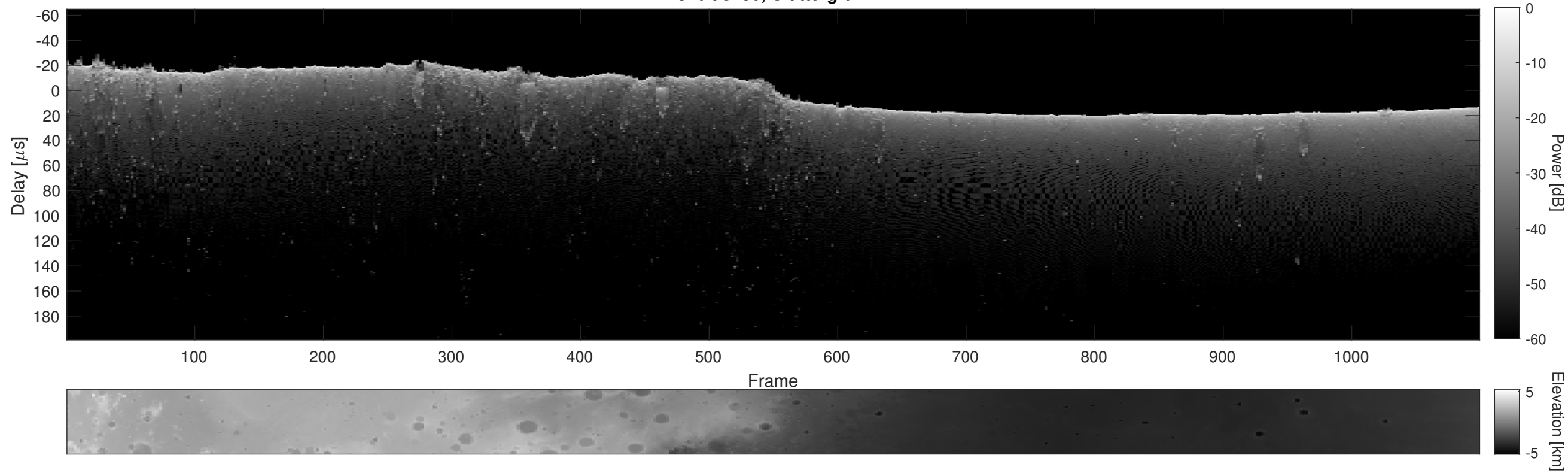
Orbit 8186, Cluttergram
