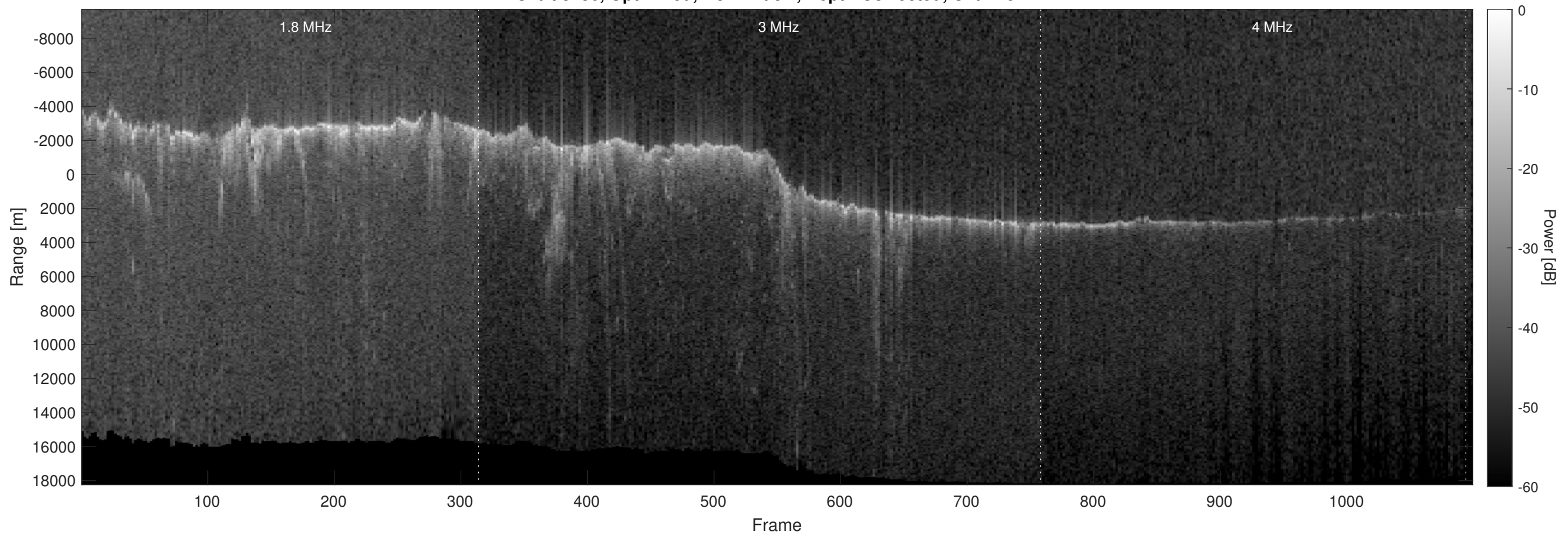
Orbit 8186, Optimized, No Window, Depth-Corrected, Channel 2
