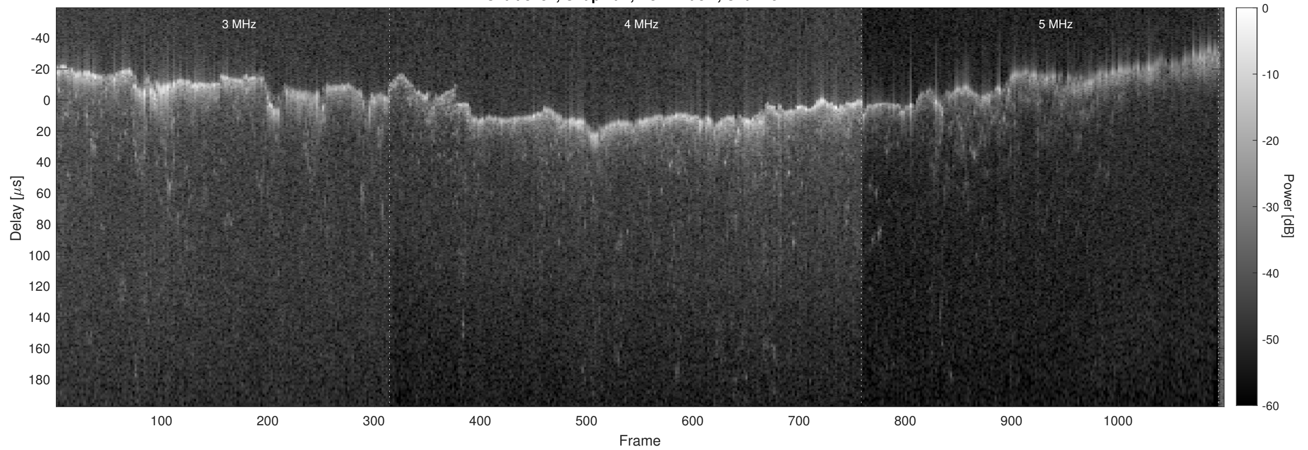
Orbit 8187, Chapman, No Window, Channel 2
