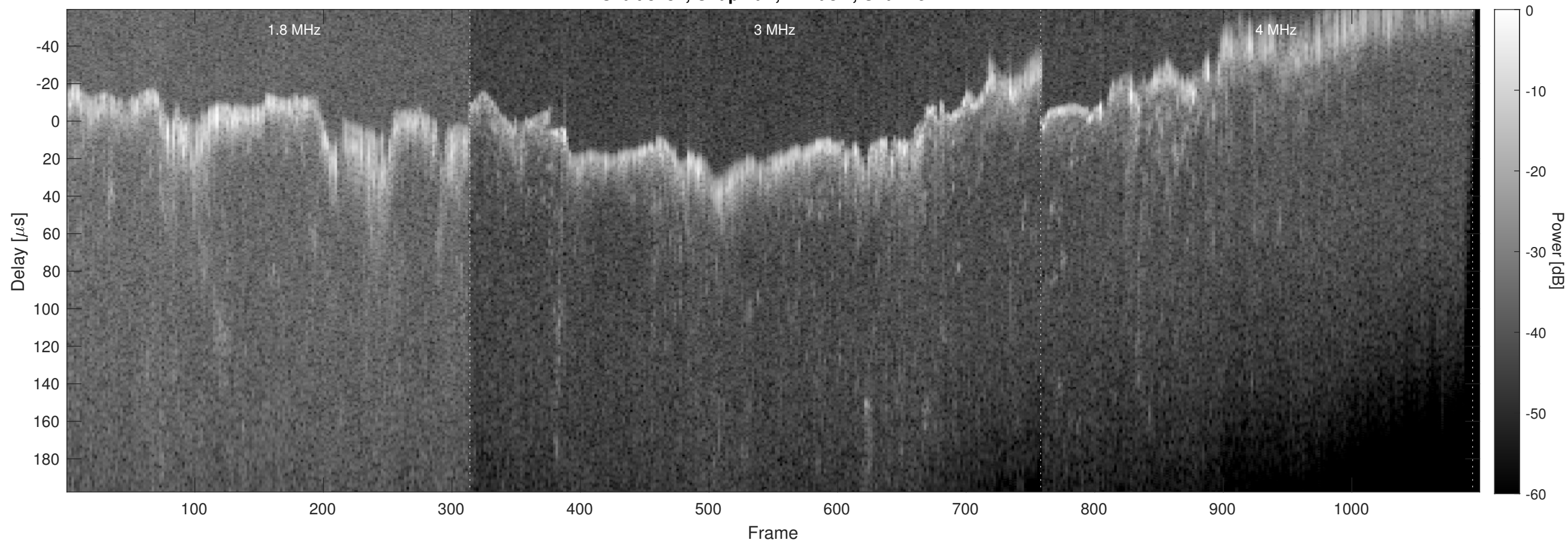
Orbit 8187, Chapman, Window, Channel 2
