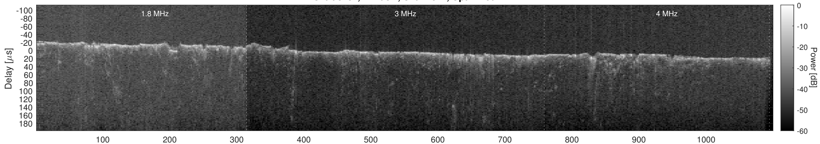
Orbit 8187, Cluttergram
