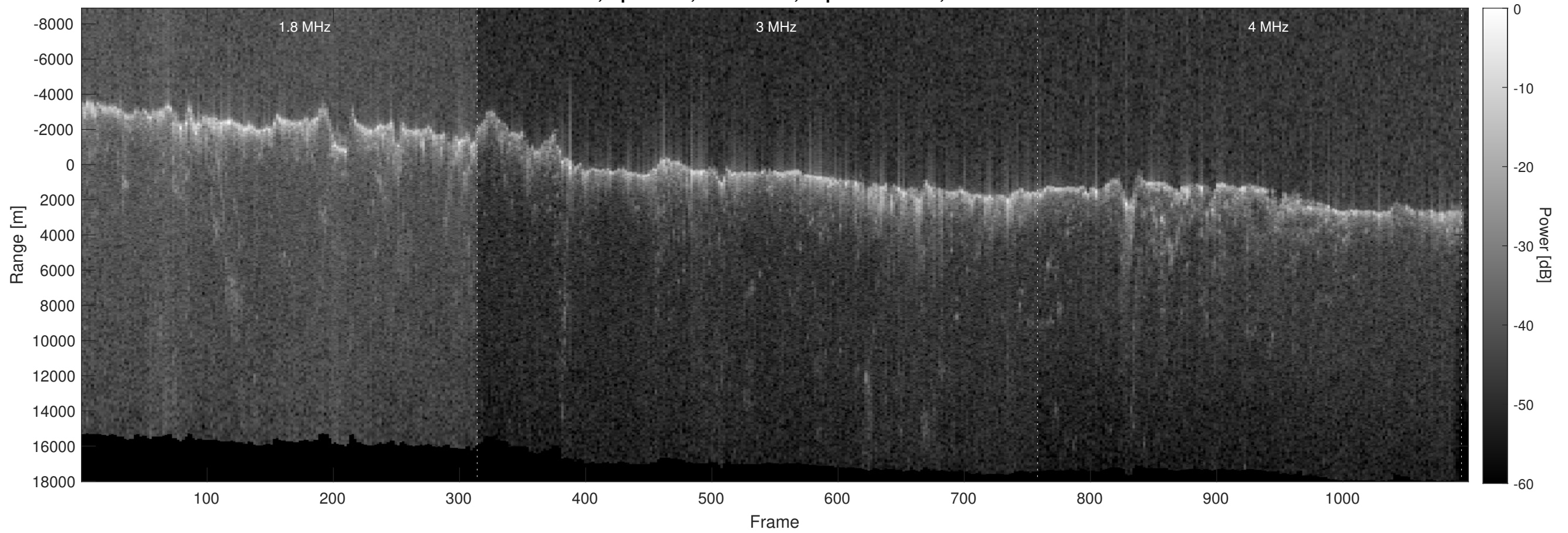
Orbit 8187, Optimized, No Window, Depth-Corrected, Channel 2
