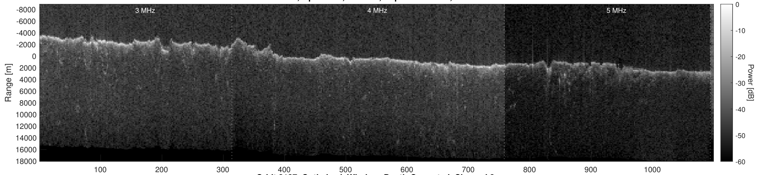
Orbit 8187, Optimized, Window, Depth-Corrected, Channel 2
