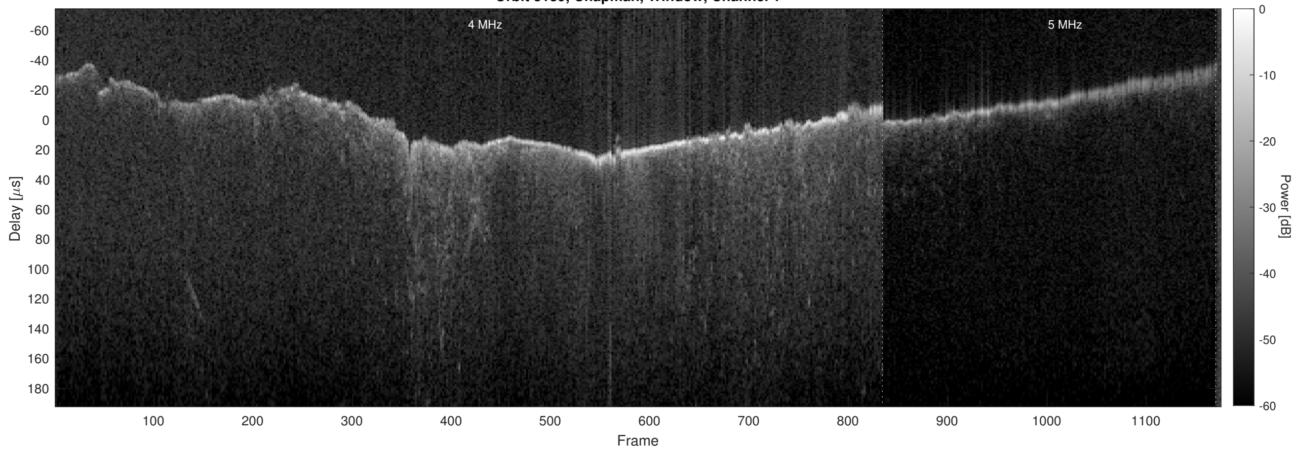
Orbit 8189, Chapman, Window, Channel 2
