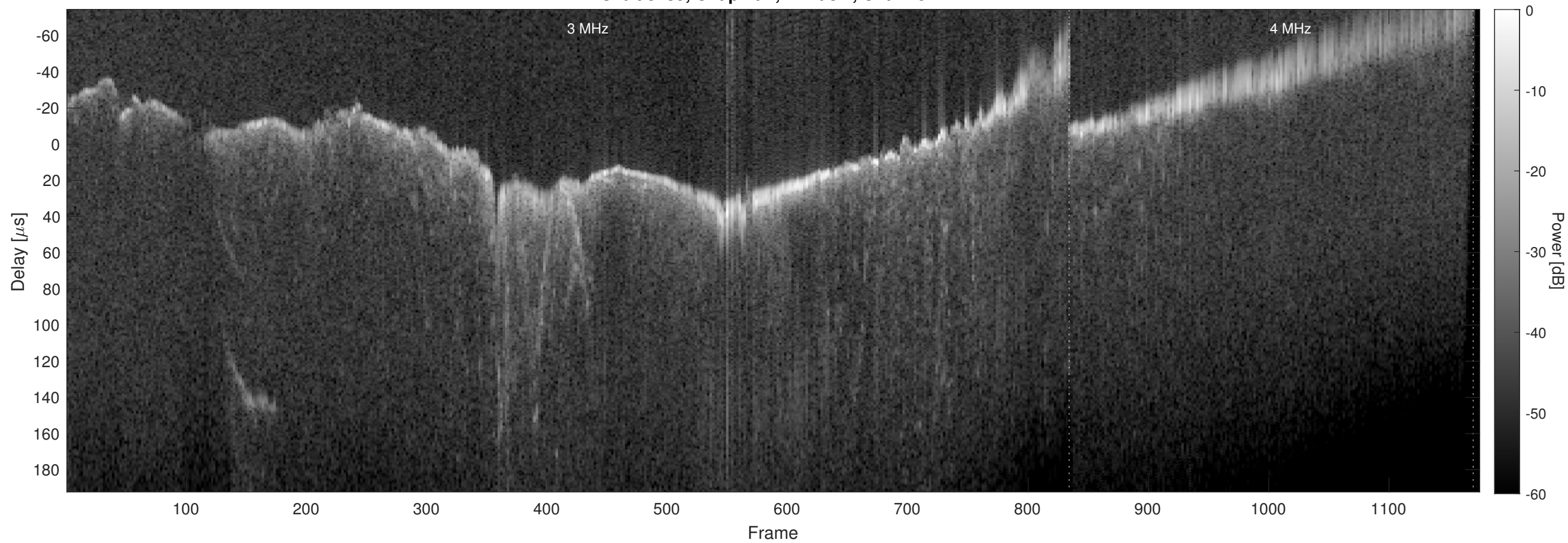
Orbit 8189, Chapman, Window, Channel 2
