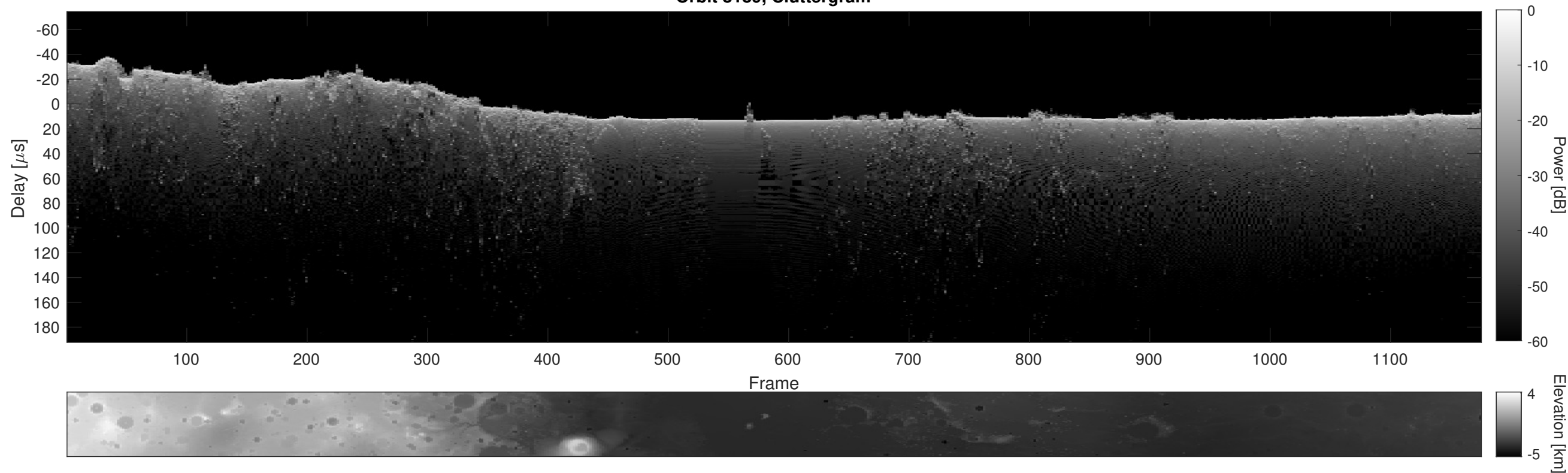
Orbit 8189, Cluttergram
