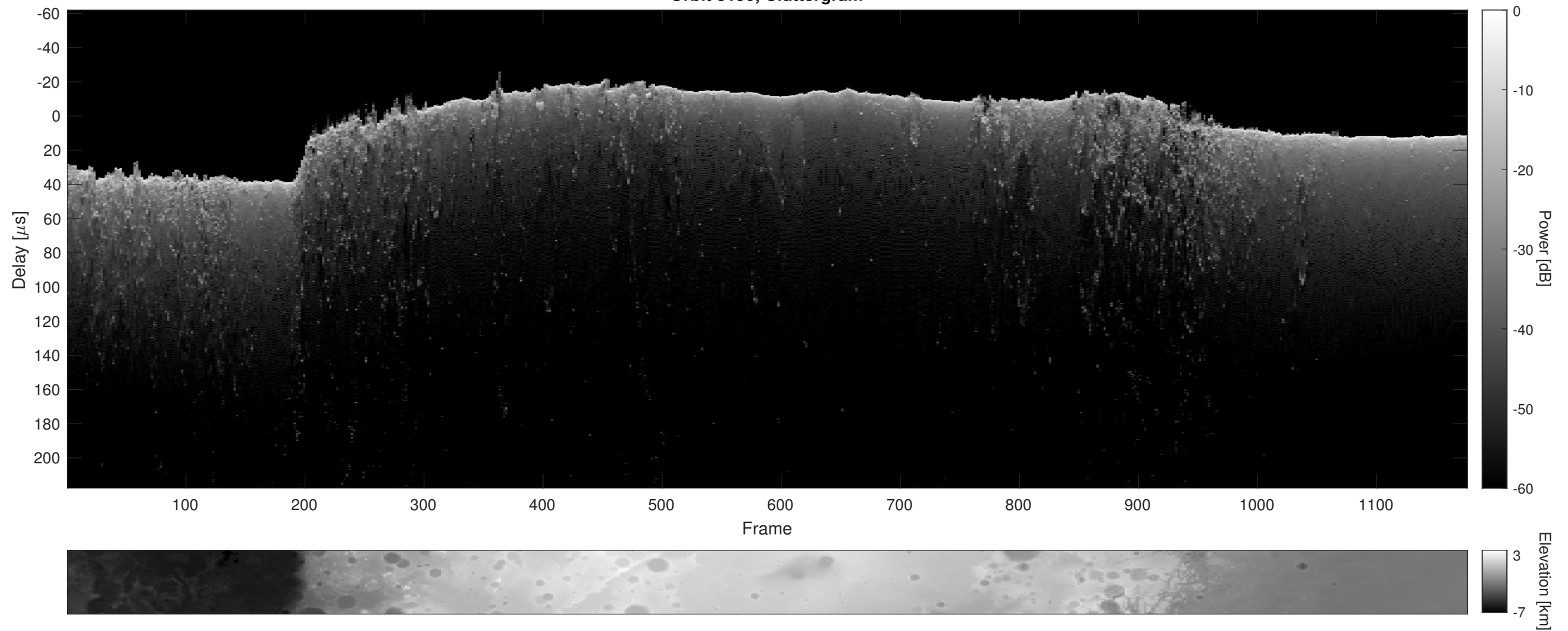
Orbit 8190, Cluttergram
