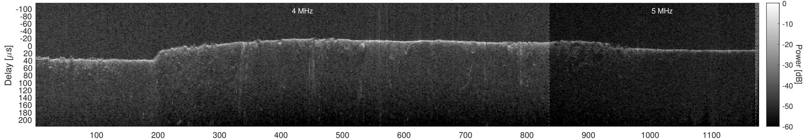
Orbit 8190, Cluttergram
