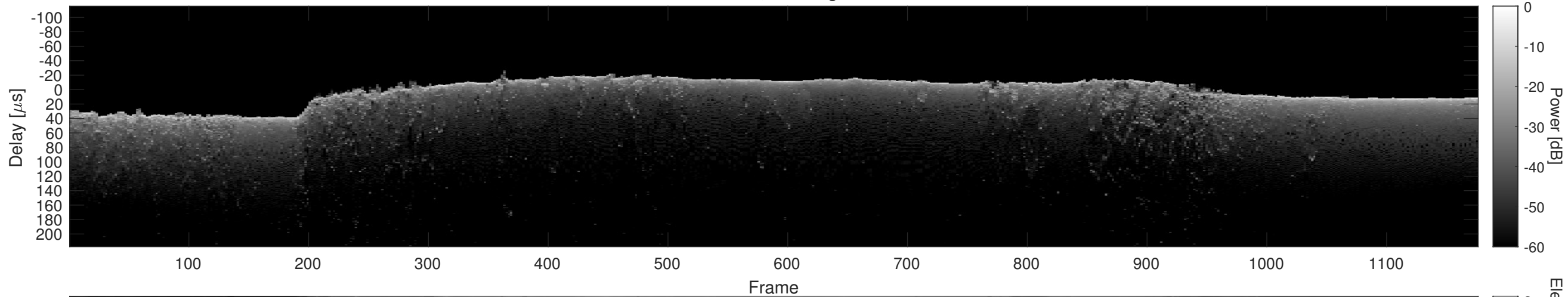
Orbit 8190, Cluttergram
