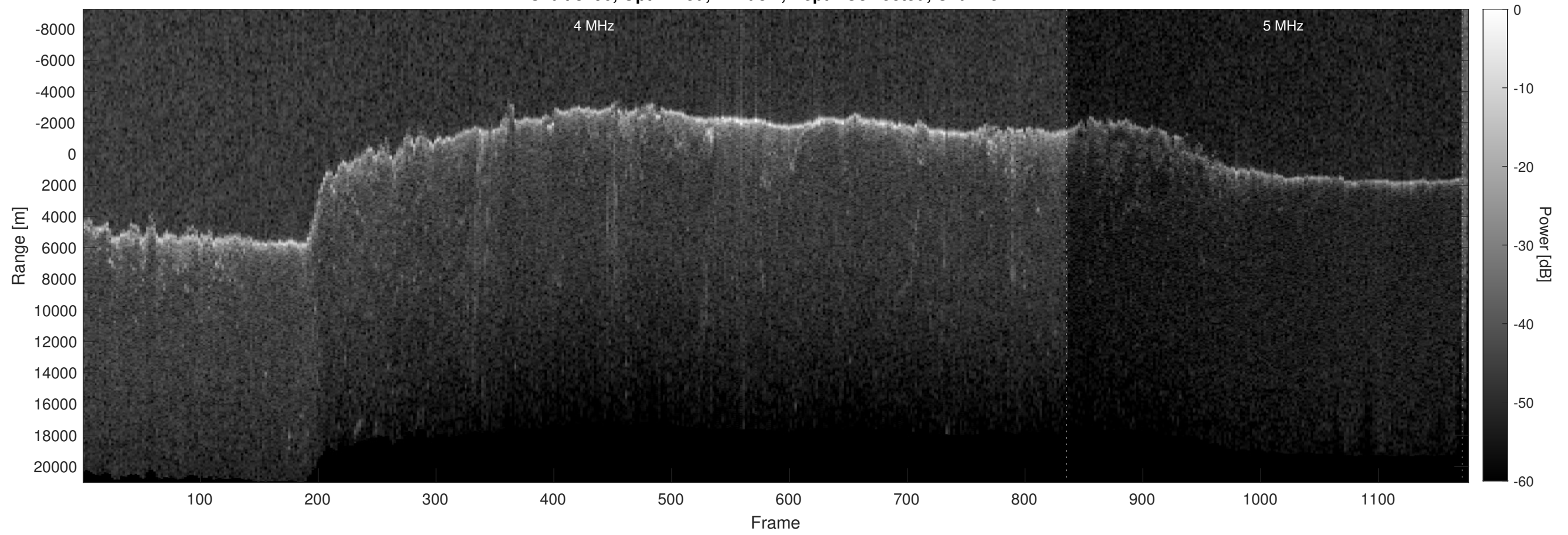
Orbit 8190, Optimized, Window, Depth-Corrected, Channel 2
