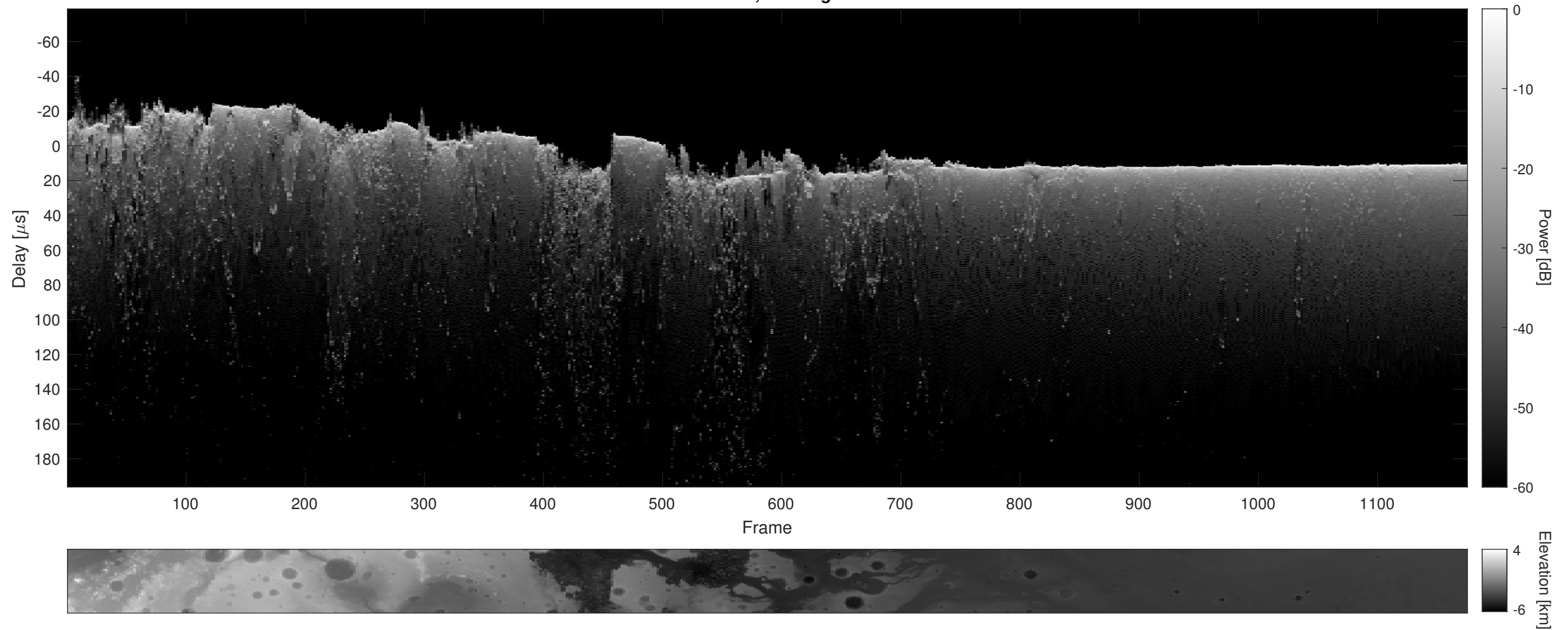
Orbit 8191, Cluttergram
