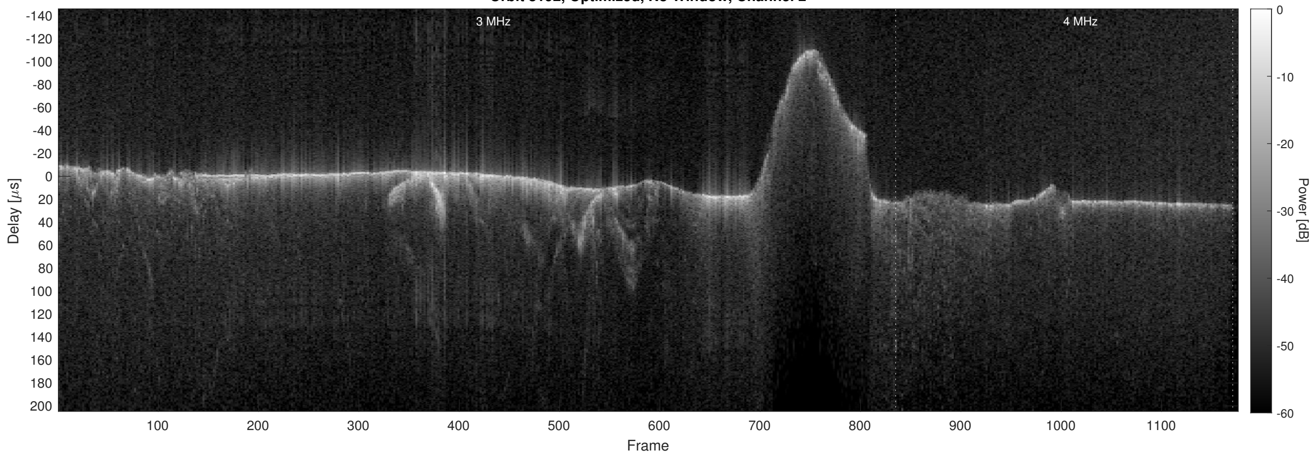
Orbit 8192, Optimized, No Window, Channel 2
