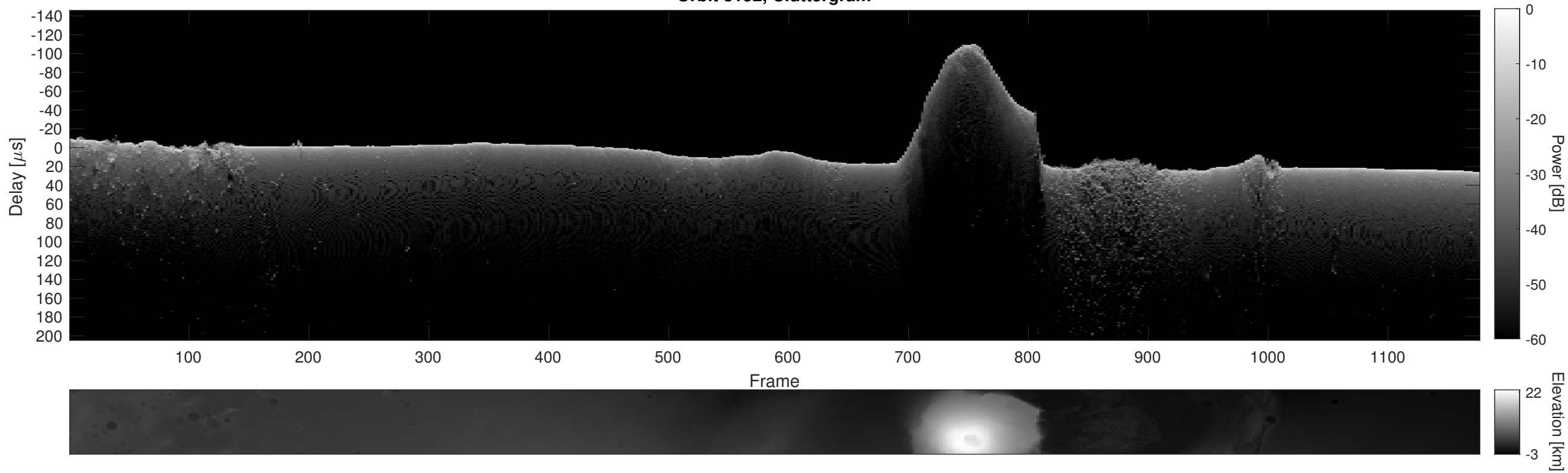
Orbit 8192, Cluttergram
