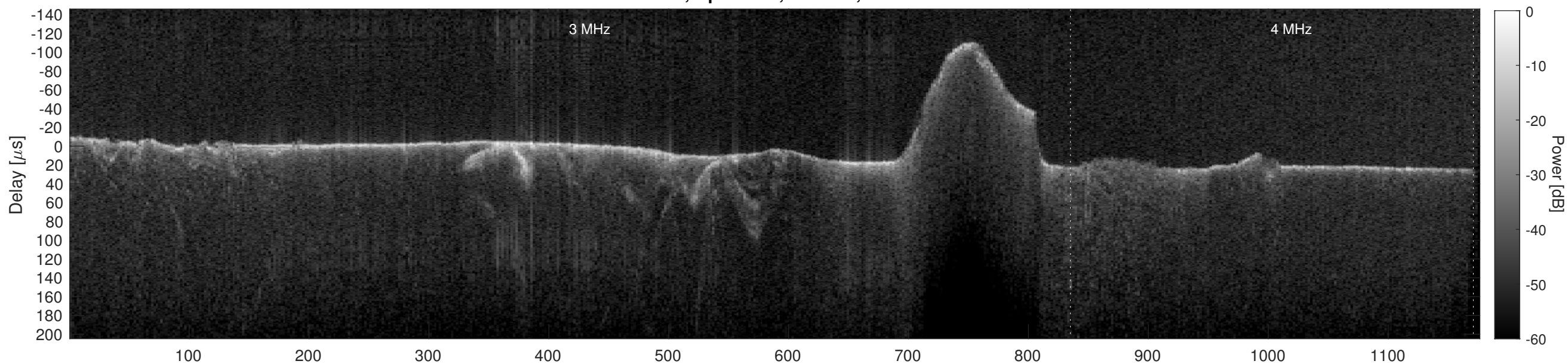
Orbit 8192, Cluttergram
