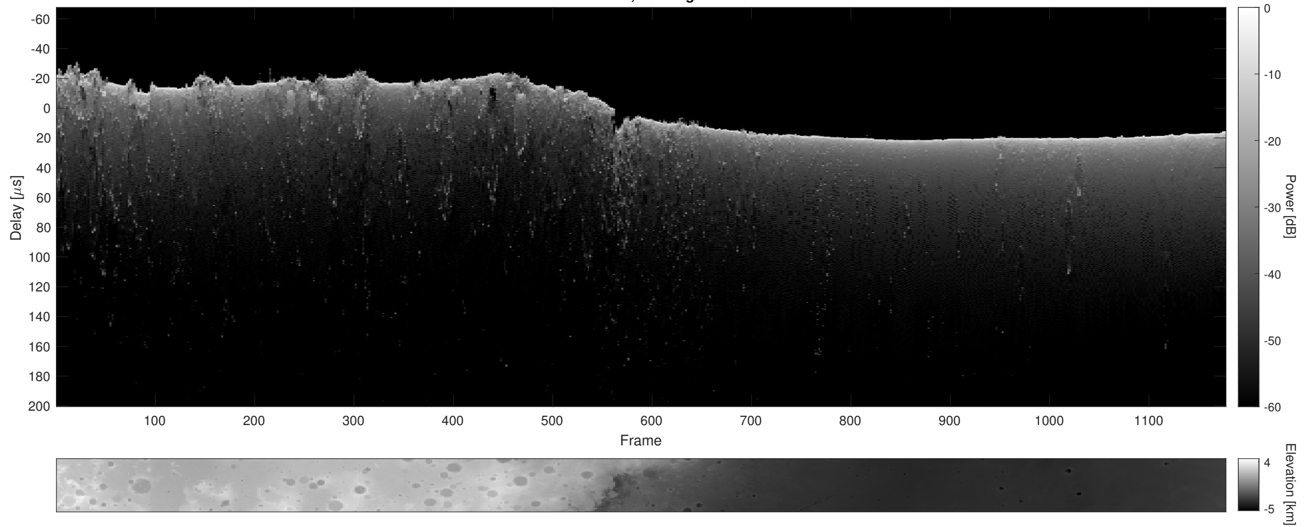
Orbit 8193, Cluttergram
