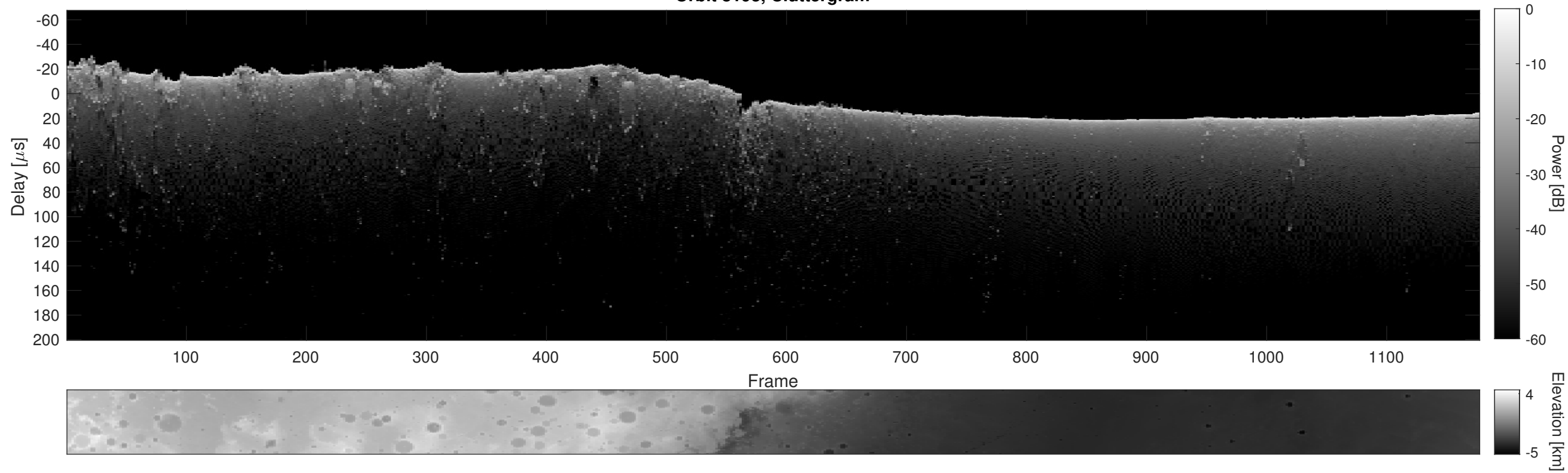
Orbit 8193, Cluttergram
