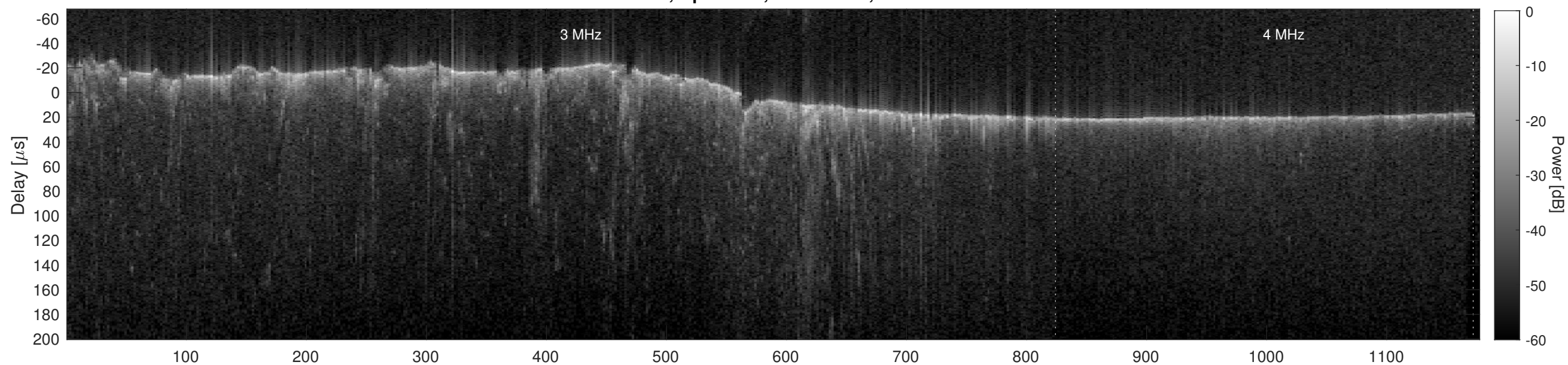
Orbit 8193, Cluttergram
