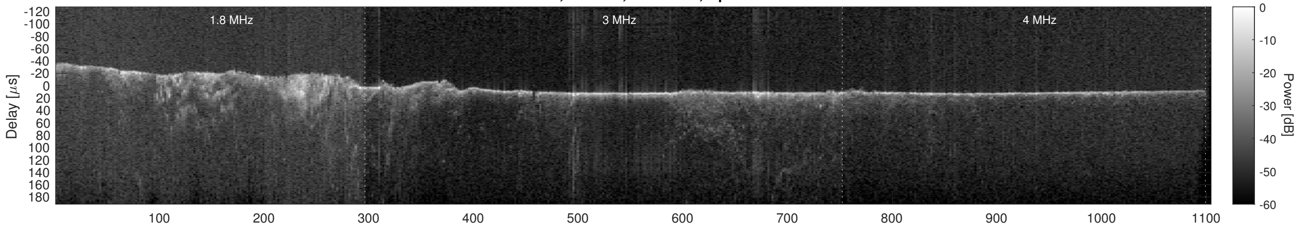
Orbit 8196, Cluttergram
