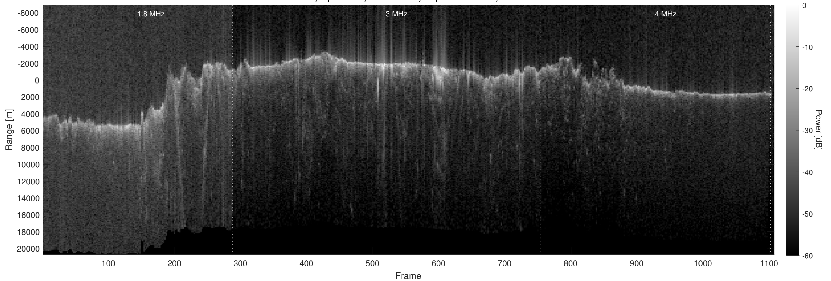
Orbit 8197, Optimized, No Window, Depth-Corrected, Channel 2
