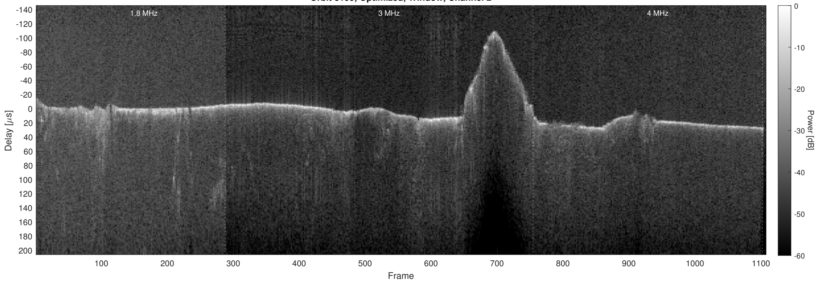
Orbit 8199, Optimized, Window, Channel 2
