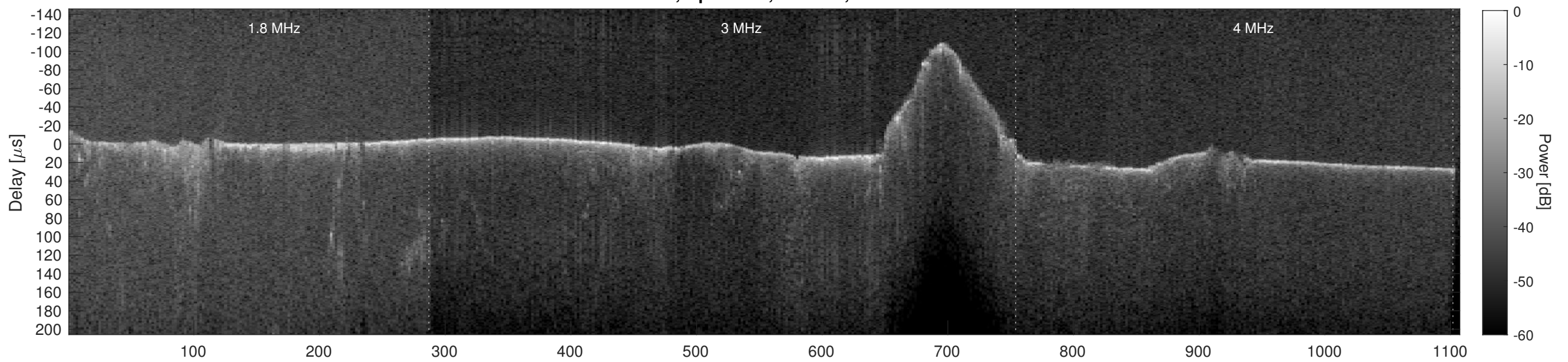
Orbit 8199, Cluttergram
