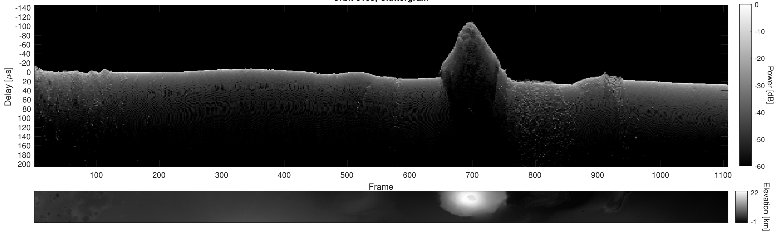
Orbit 8199, Cluttergram
