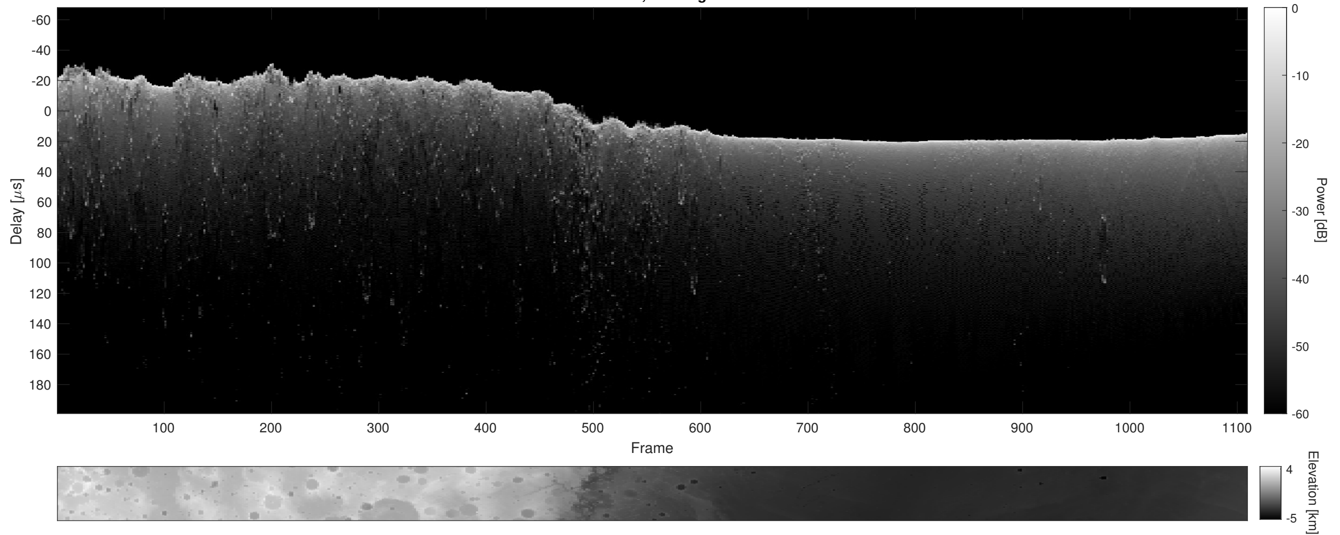
Orbit 8200, Cluttergram
