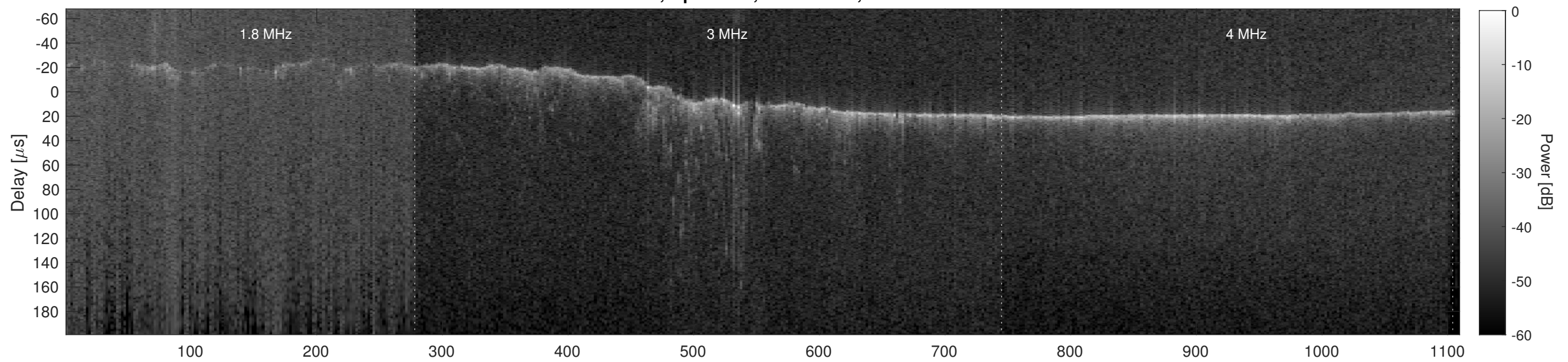
Orbit 8200, Cluttergram
