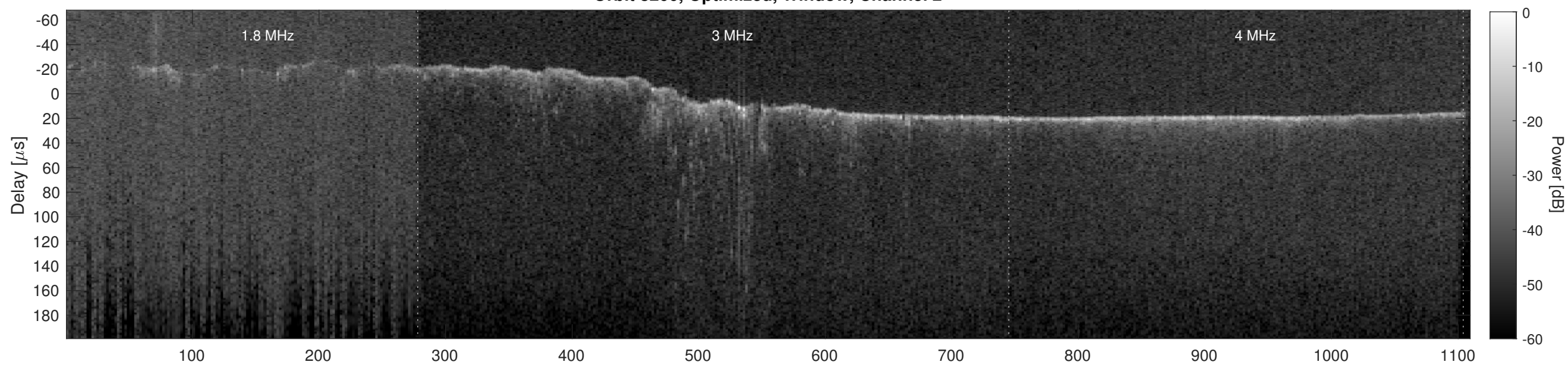
Orbit 8200, Cluttergram
