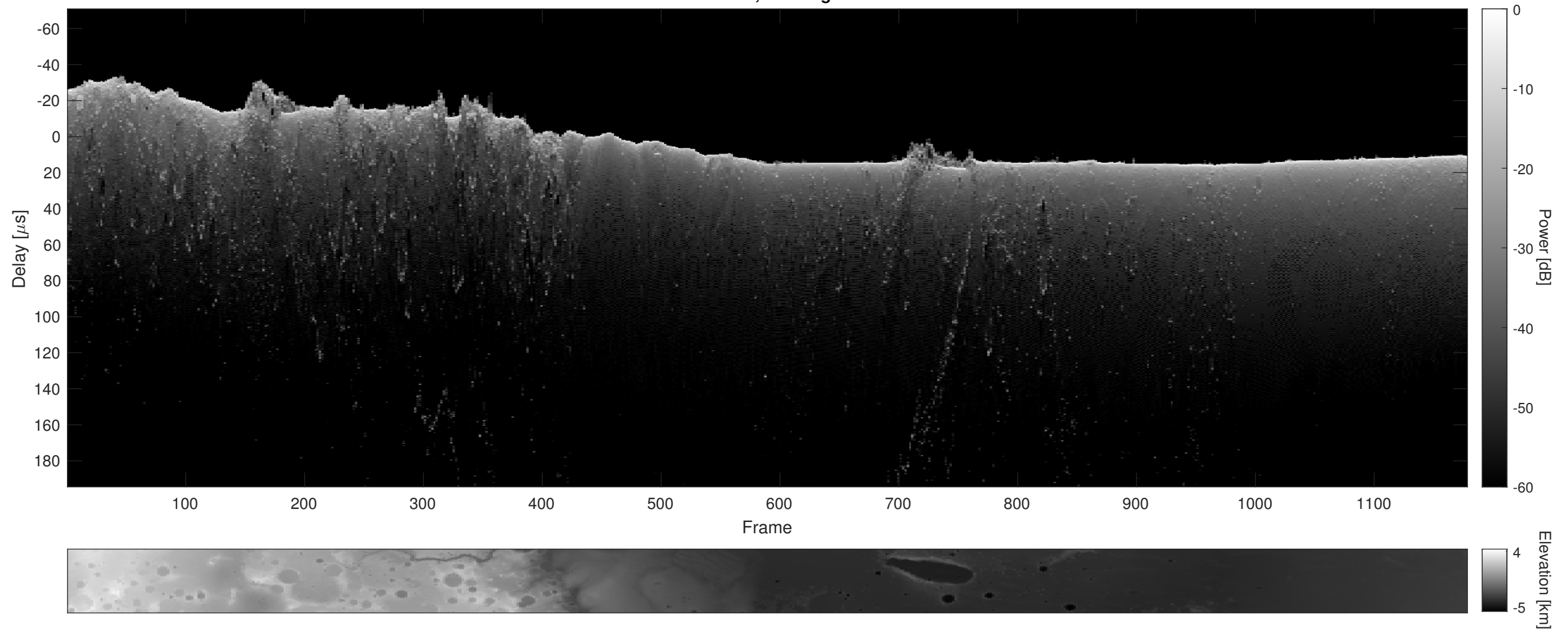
Orbit 8203, Cluttergram
