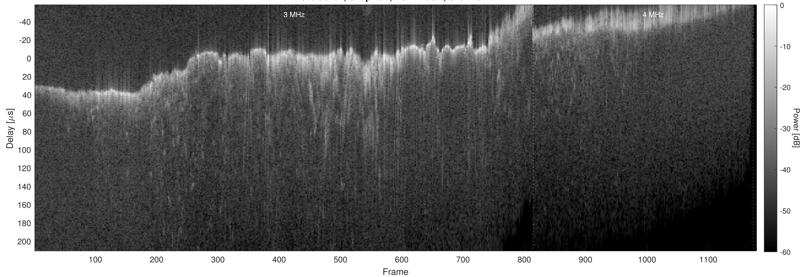
Orbit 8204, Chapman, No Window, Channel 2
