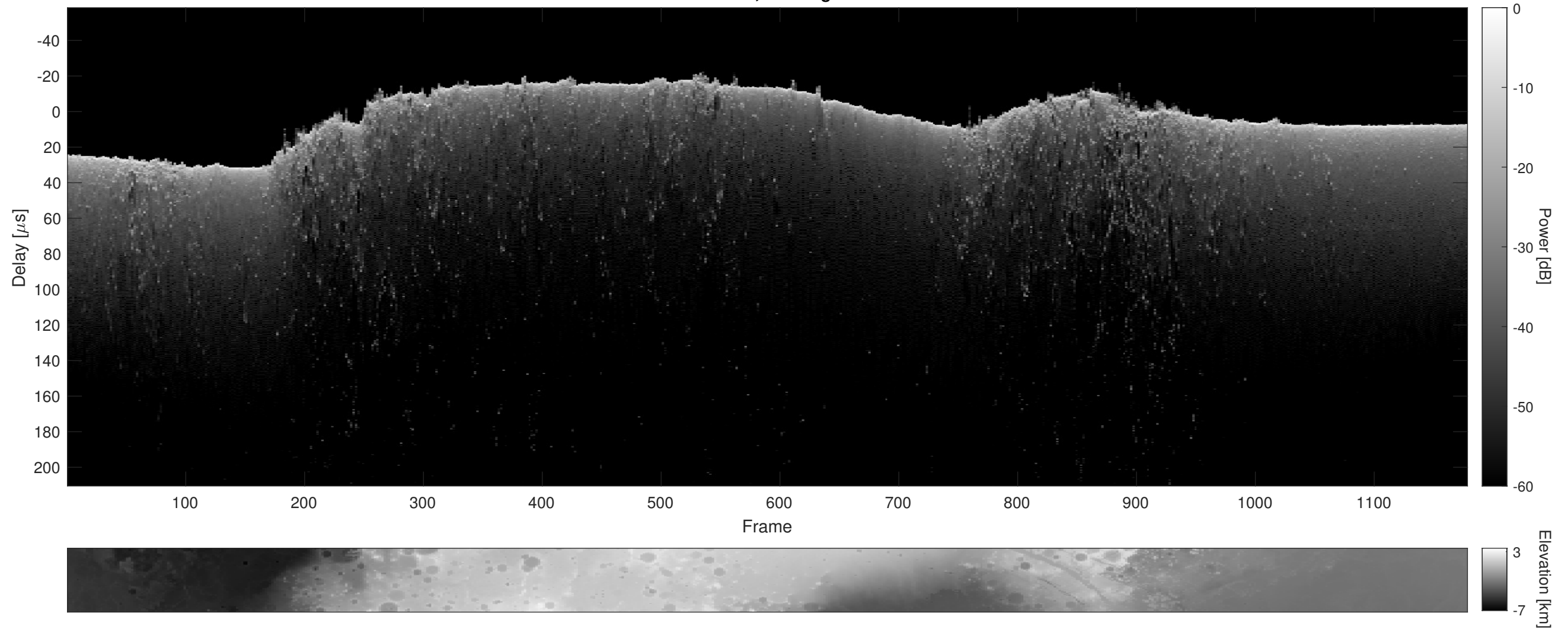
Orbit 8204, Cluttergram
