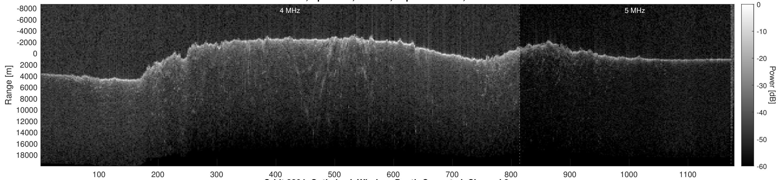
Orbit 8204, Optimized, Window, Depth-Corrected, Channel 2
