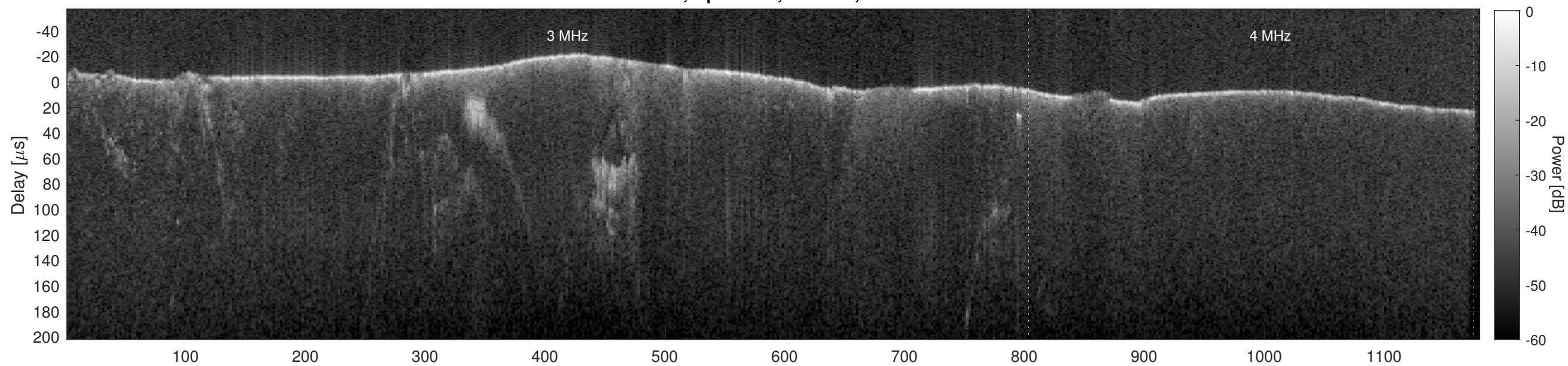
Orbit 8206, Cluttergram
