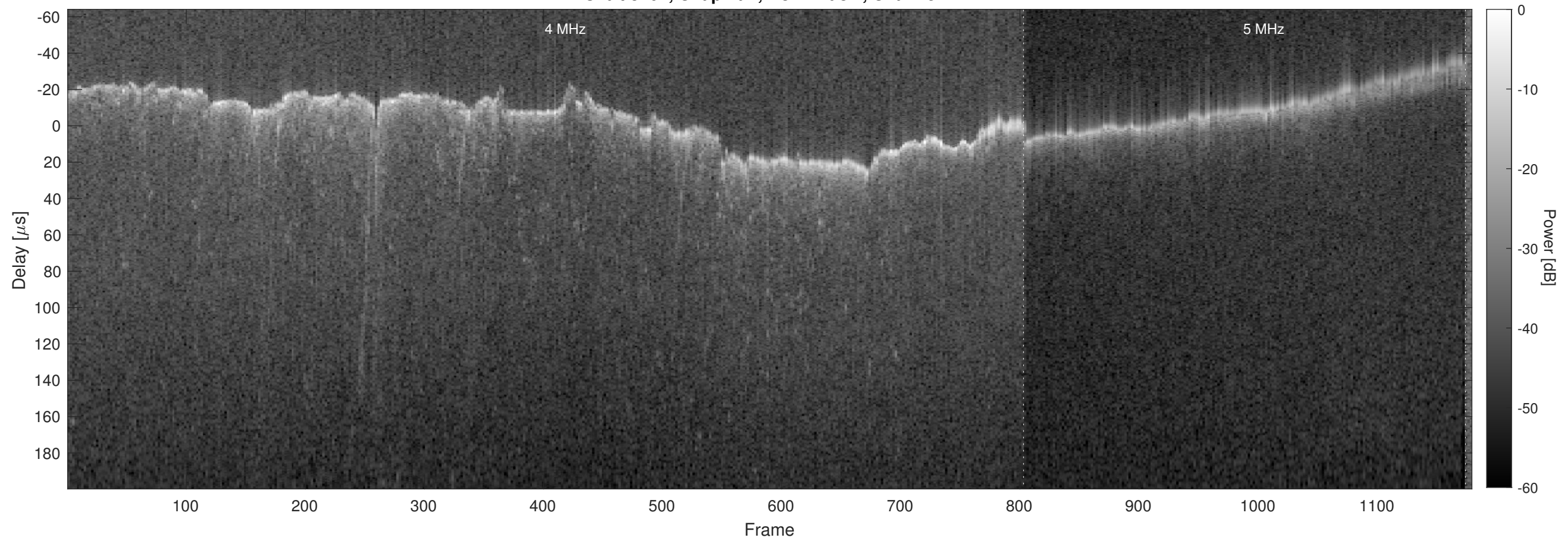
Orbit 8207, Chapman, No Window, Channel 2
