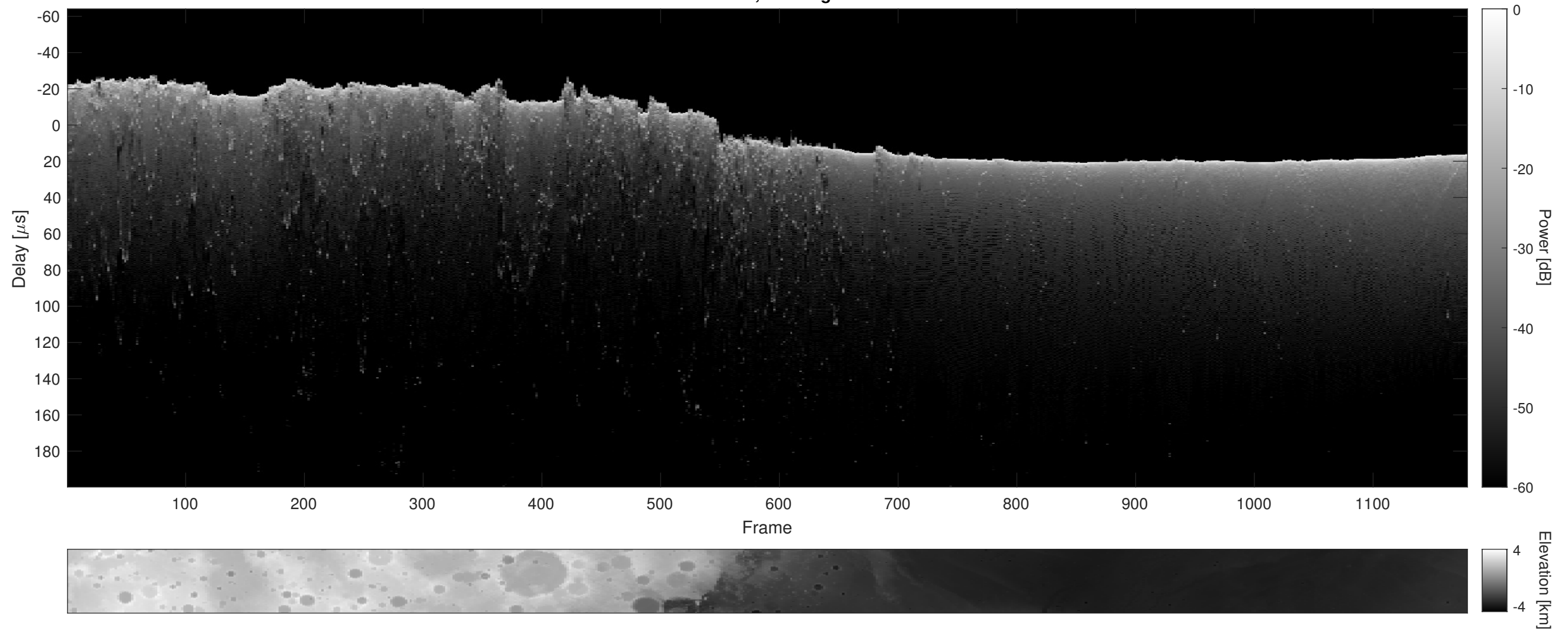
Orbit 8207, Cluttergram
