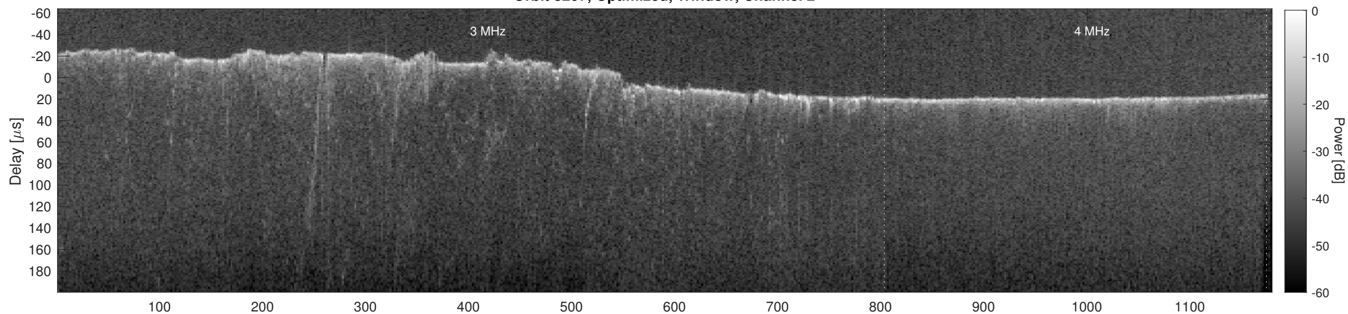
Orbit 8207, Cluttergram
