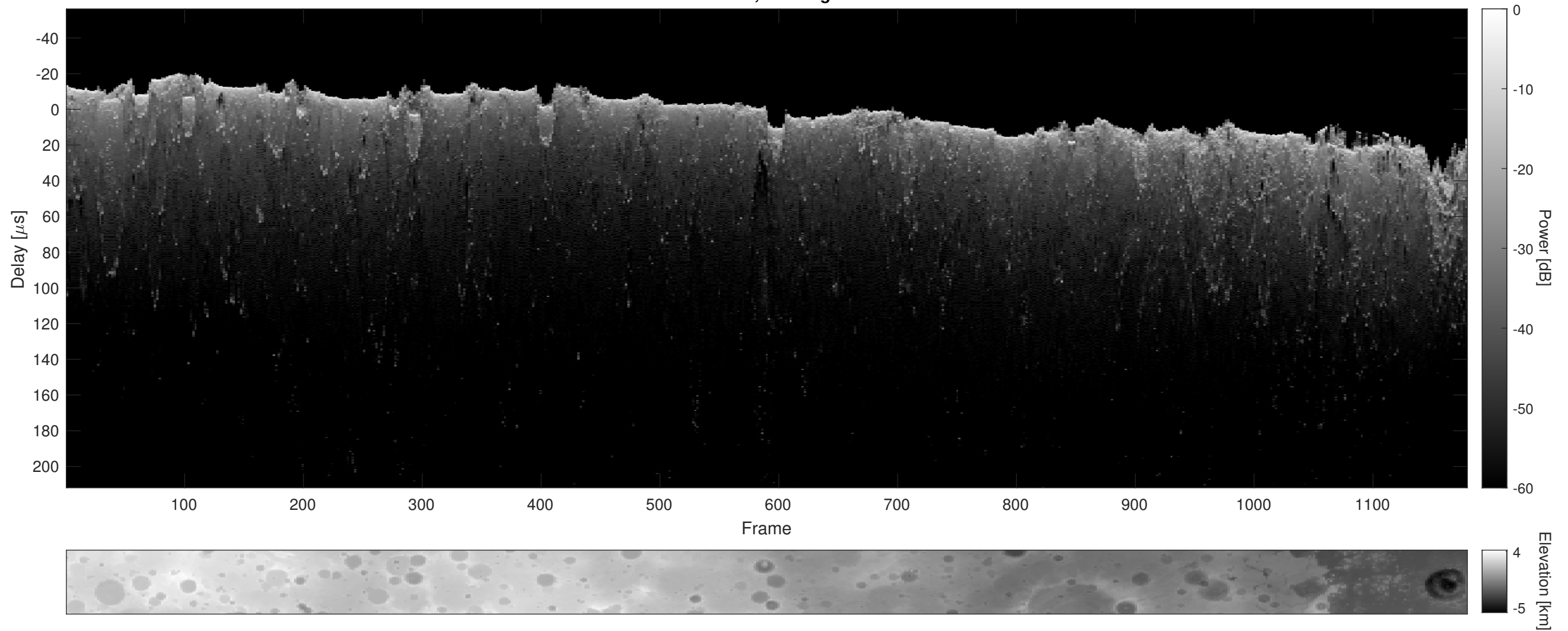
Orbit 8208, Cluttergram
