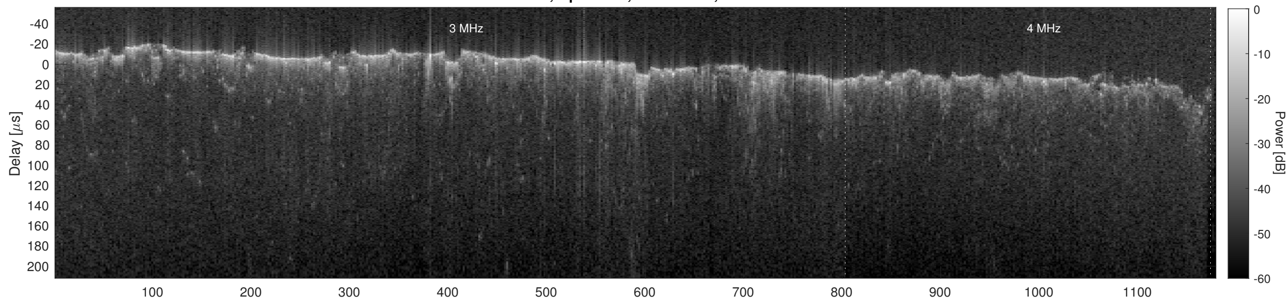
Orbit 8208, Cluttergram
