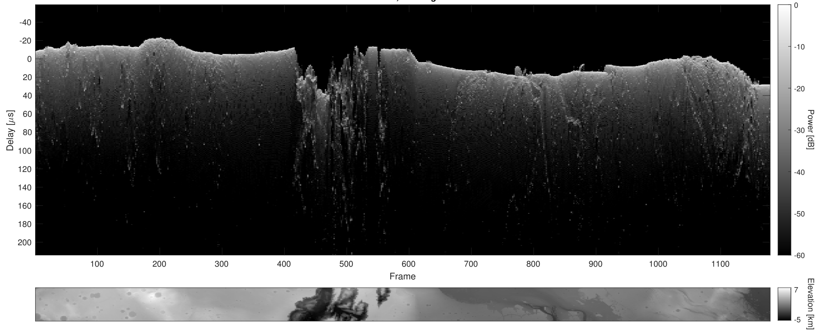
Orbit 8209, Cluttergram
