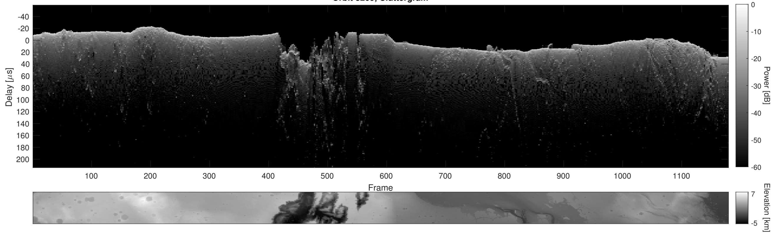
Orbit 8209, Cluttergram
