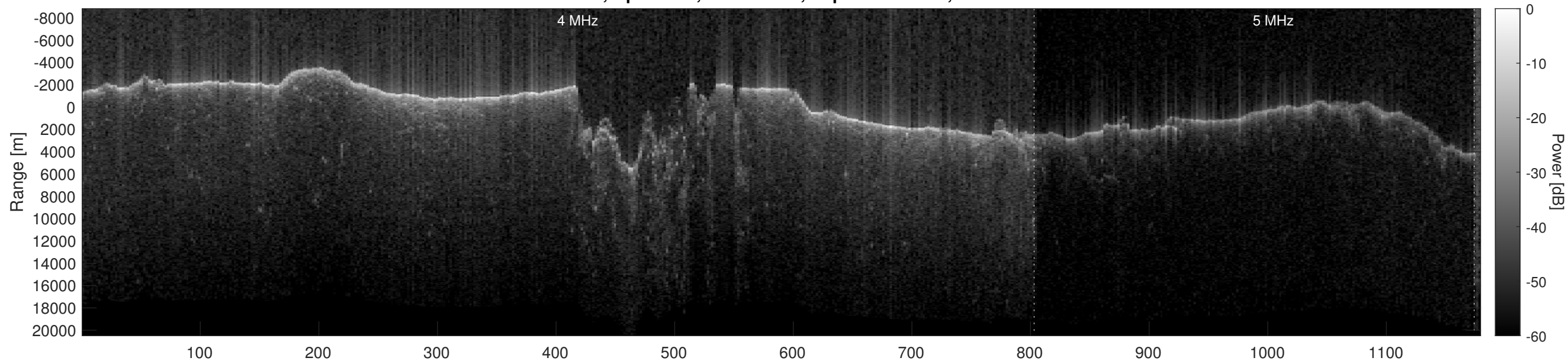
Orbit 8209, Optimized, No Window, Depth-Corrected, Channel 2
