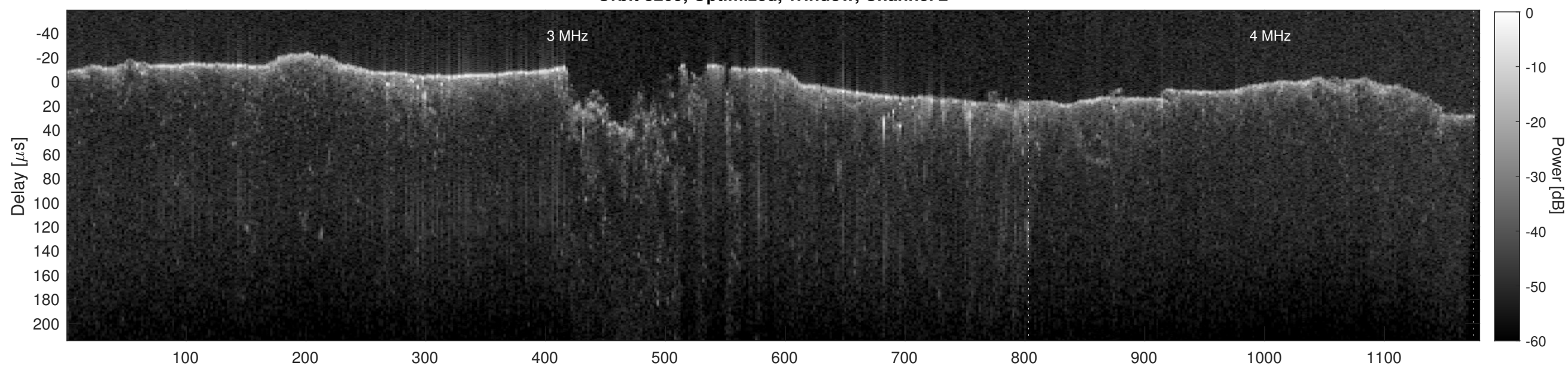
Orbit 8209, Cluttergram
