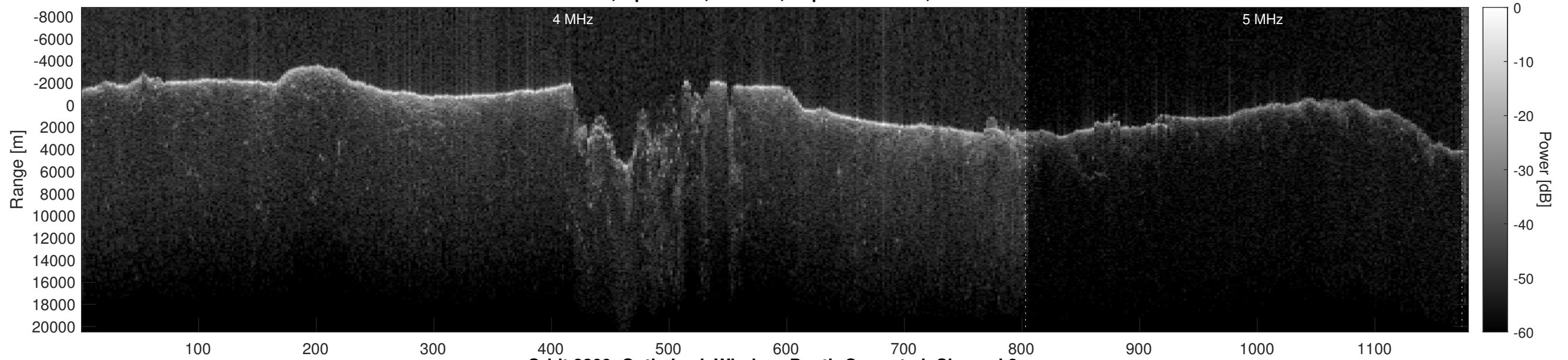
Orbit 8209, Optimized, Window, Depth-Corrected, Channel 2
