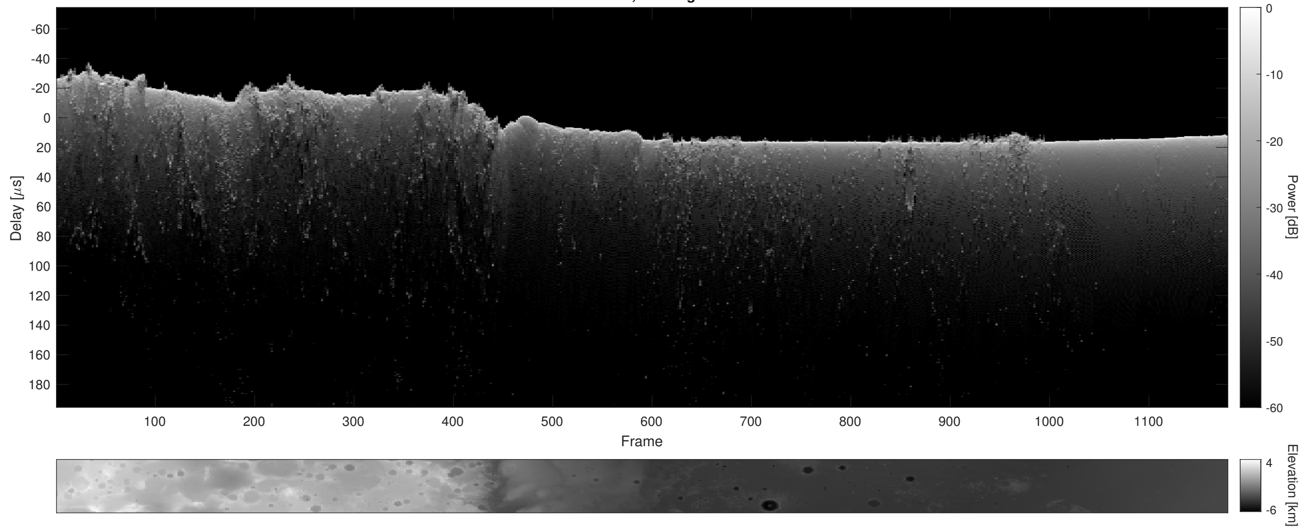
Orbit 8210, Cluttergram
