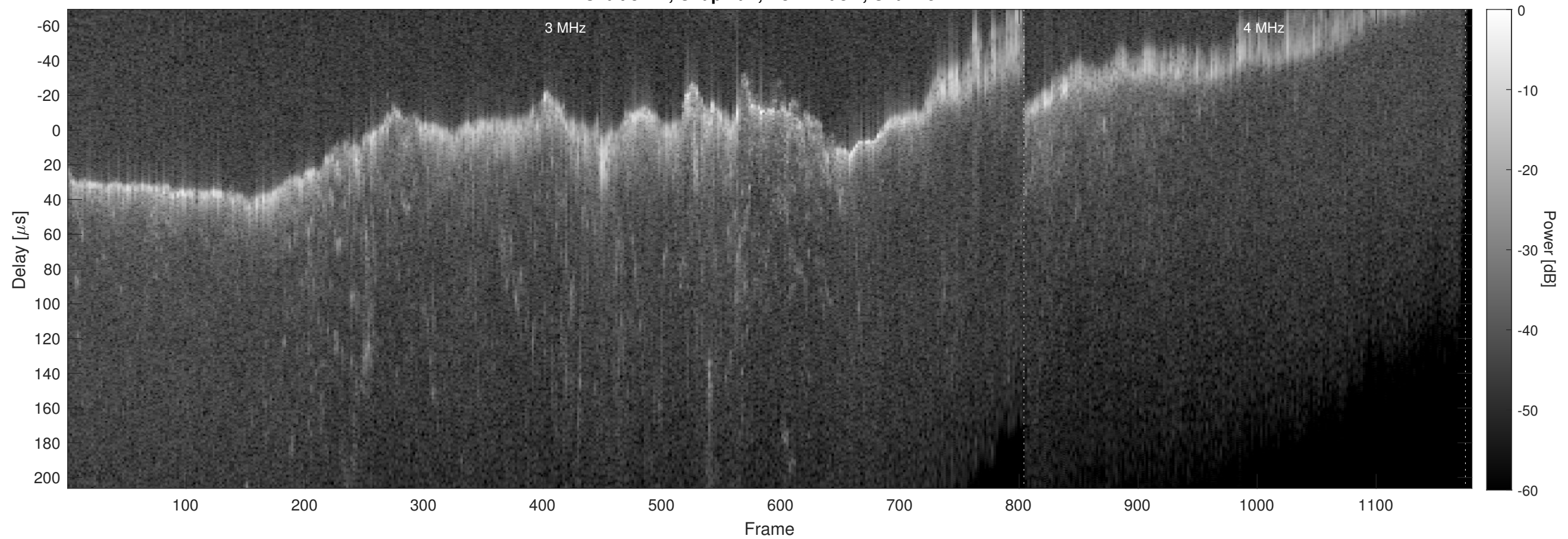
Orbit 8211, Chapman, No Window, Channel 2
