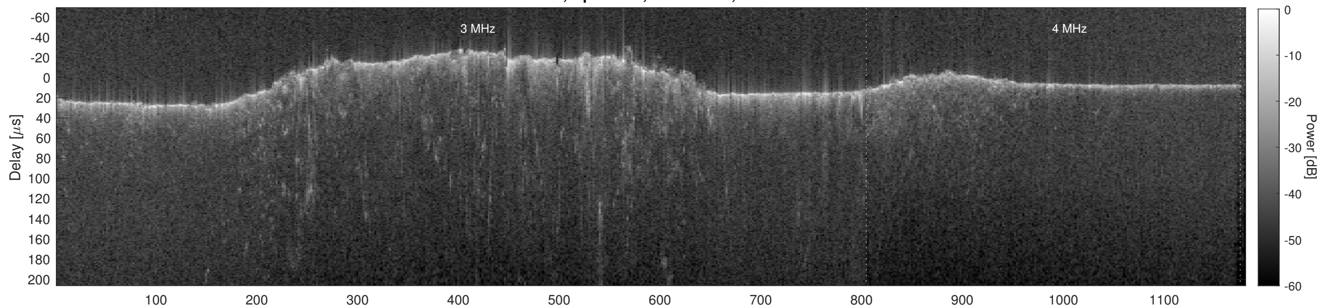
Orbit 8211, Cluttergram
