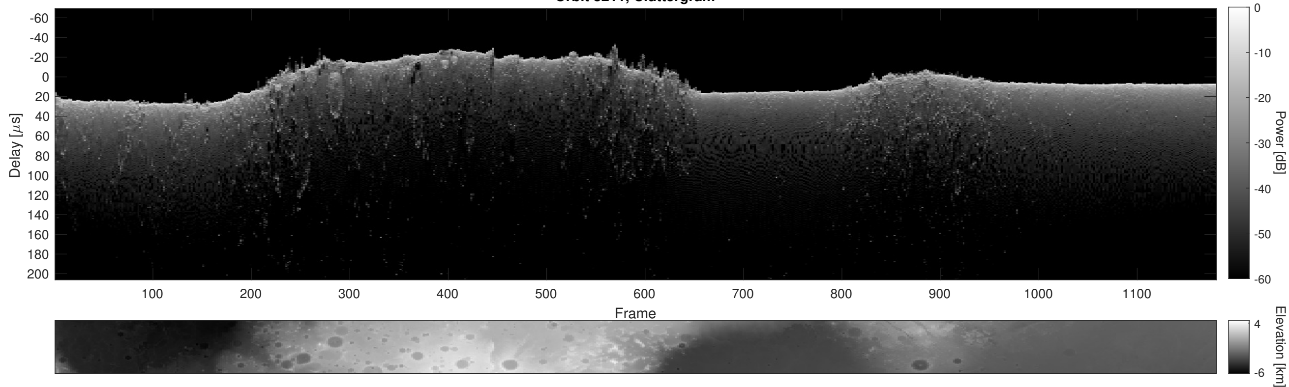
Orbit 8211, Cluttergram
