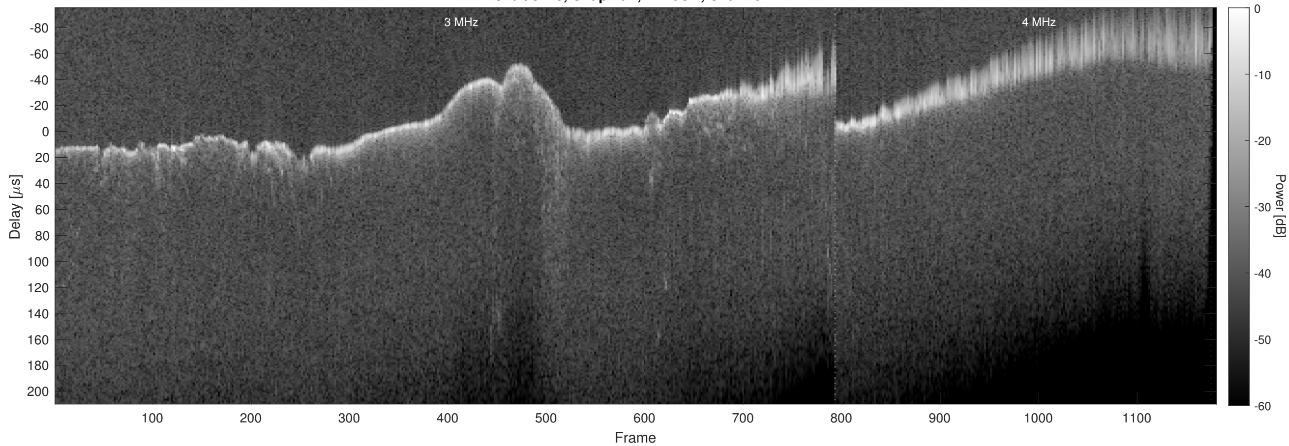
Orbit 8213, Chapman, Window, Channel 2
