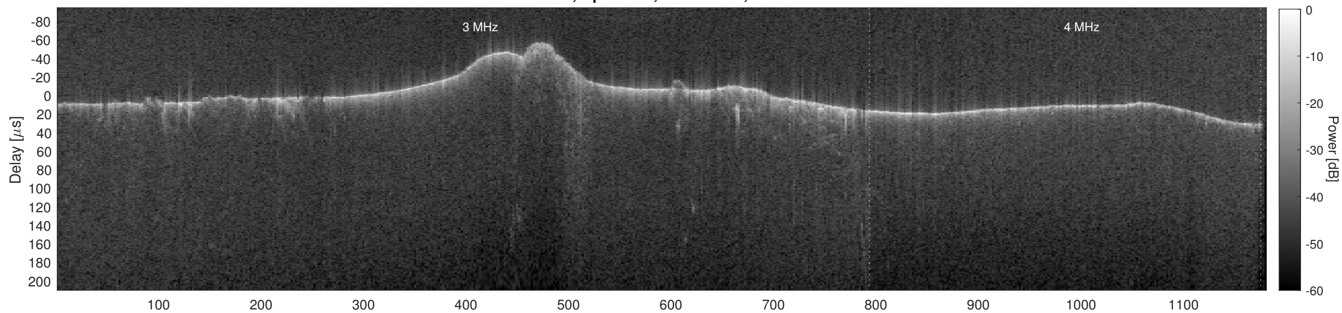
Orbit 8213, Cluttergram
