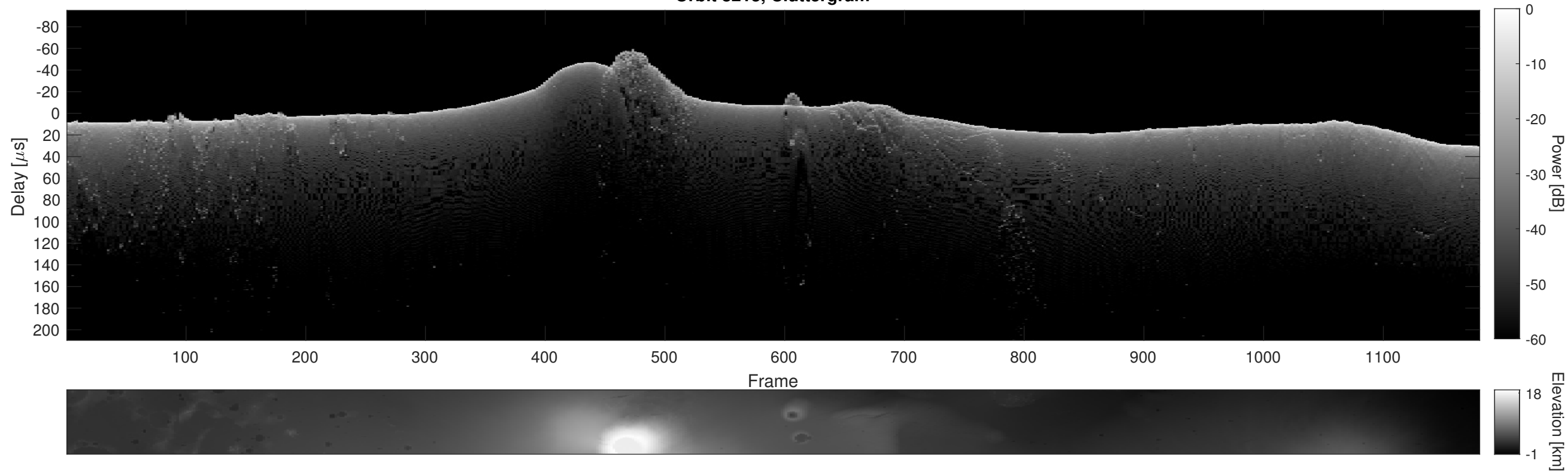
Orbit 8213, Cluttergram
