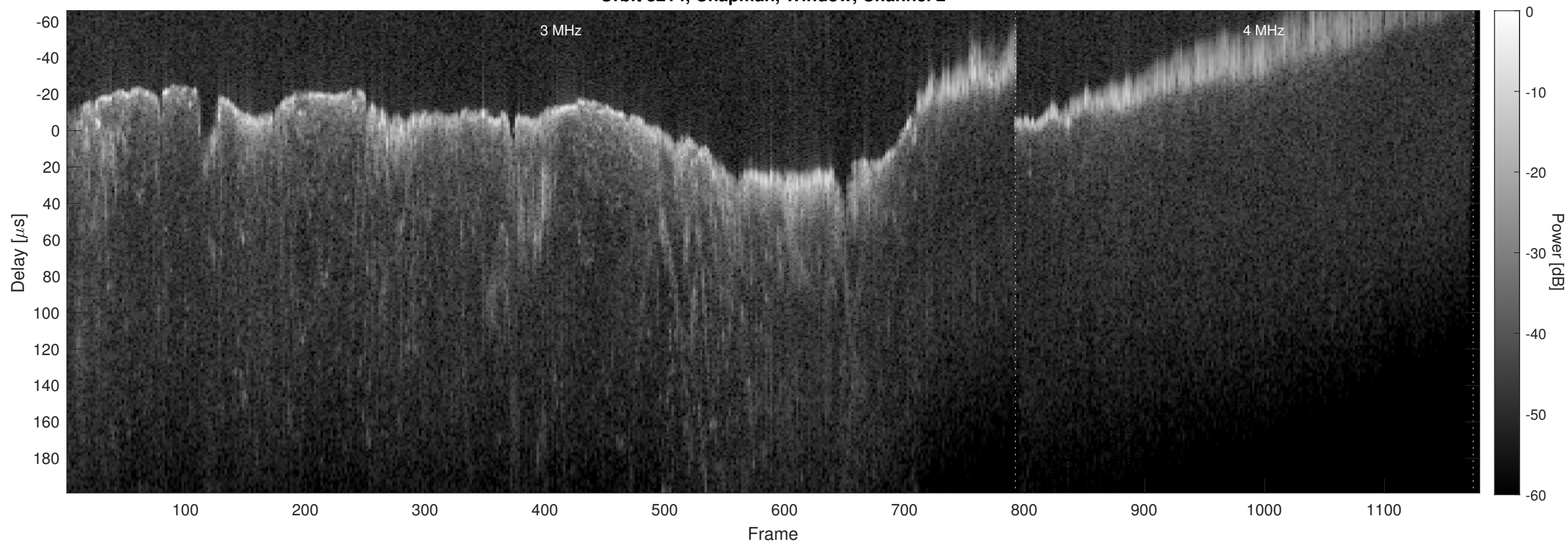
Orbit 8214, Chapman, Window, Channel 2
