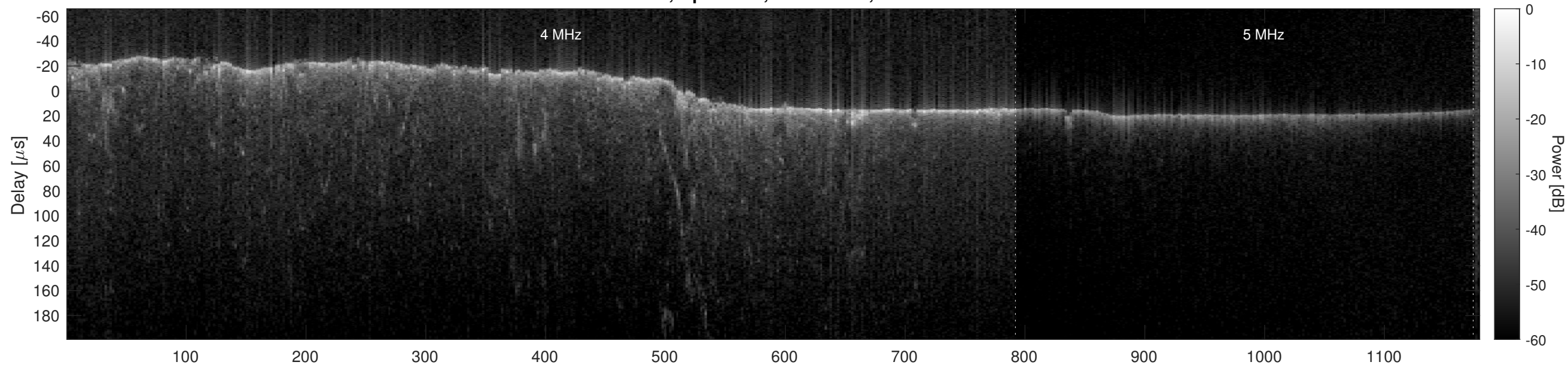
Orbit 8214, Optimized, No Window, Channel 2
