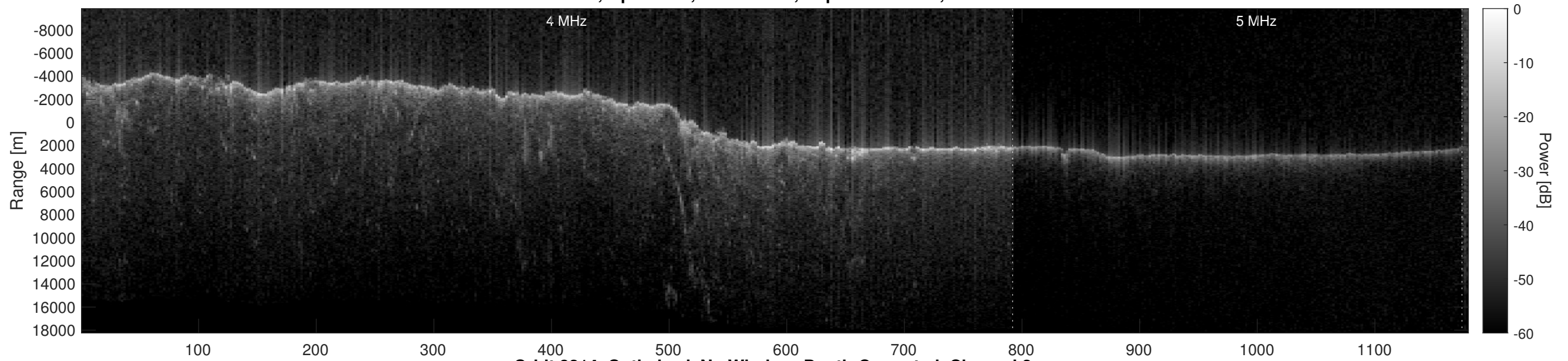
Orbit 8214, Optimized, No Window, Depth-Corrected, Channel 2
