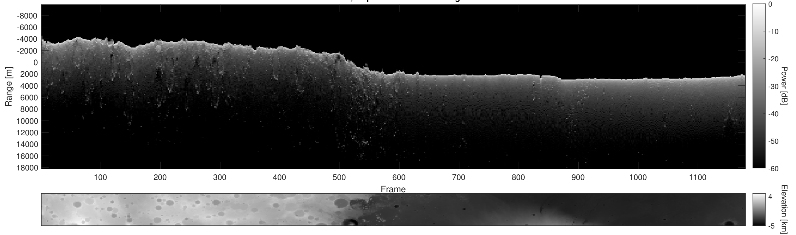
Orbit 8214, Depth-Corrected Cluttergram
