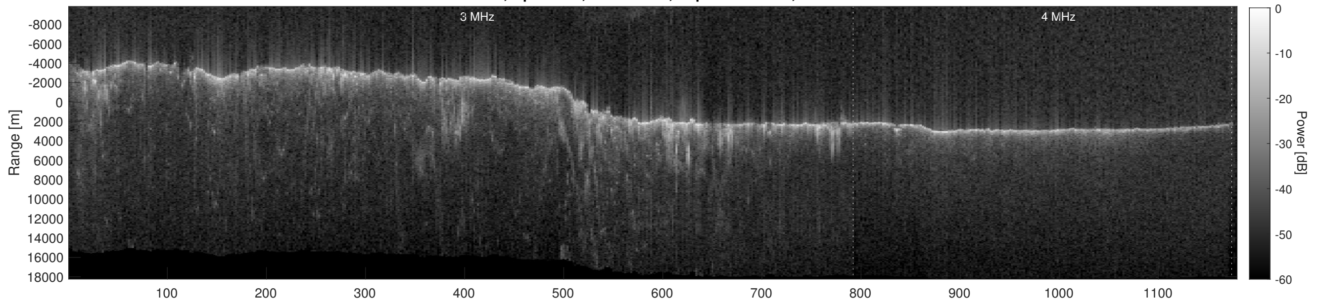
Orbit 8214, Depth-Corrected Cluttergram
