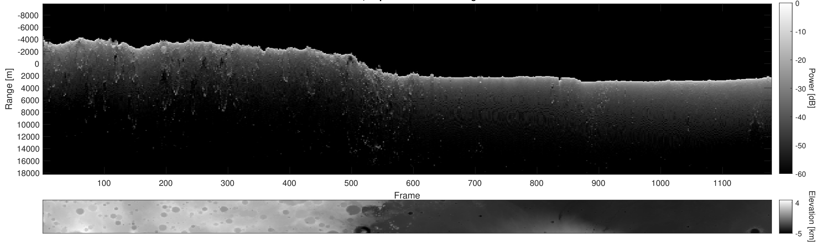
Orbit 8214, Depth-Corrected Cluttergram
