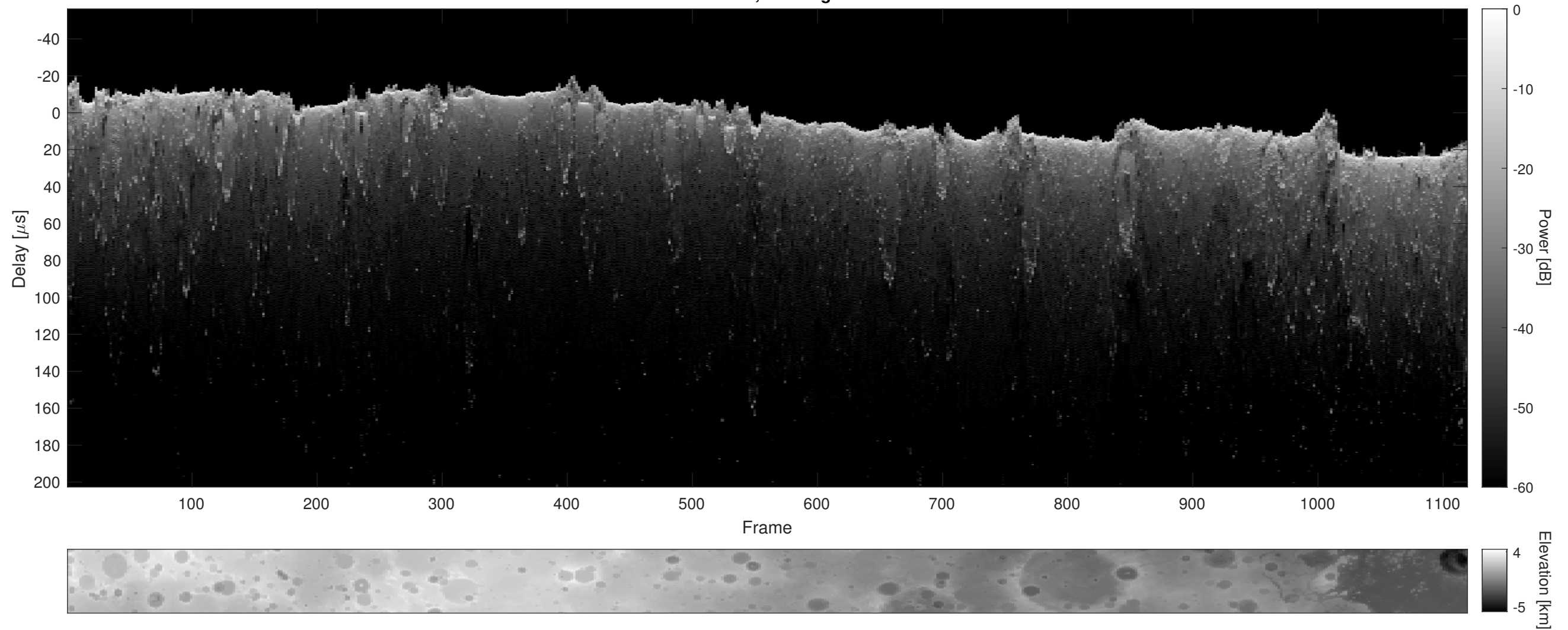
Orbit 8215, Cluttergram
